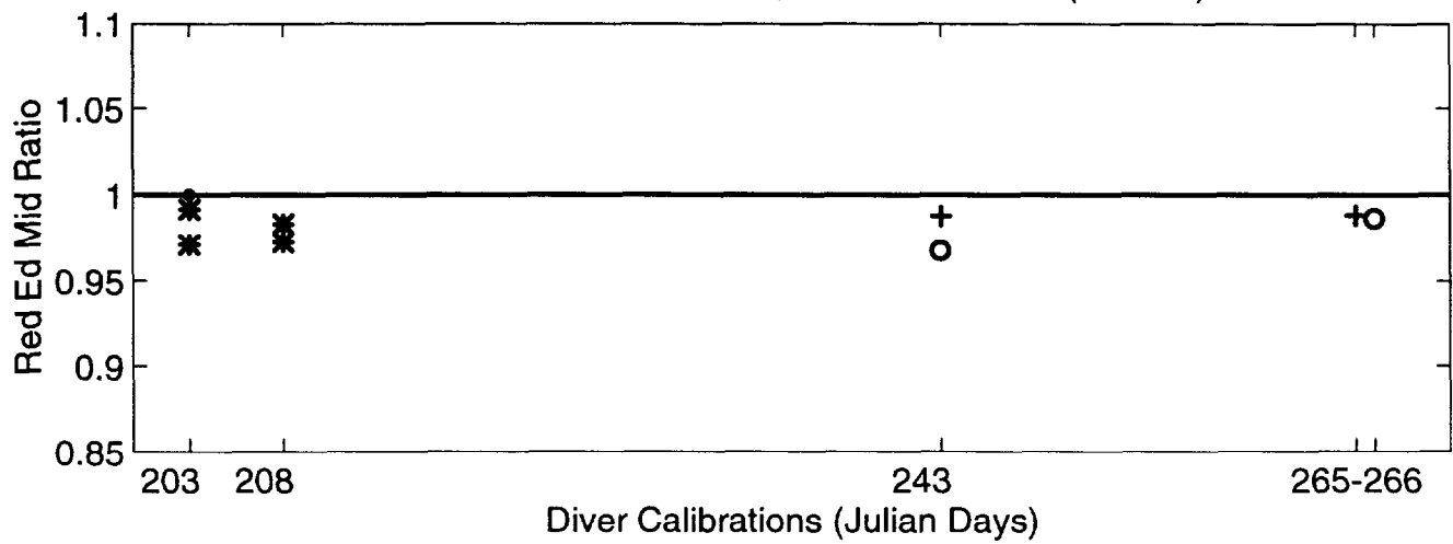
Diver Calibration - Ed Mid, SeaWifS Band 6 (670 nm)
