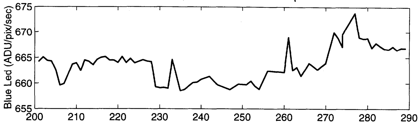
MOBY203, Maximum Blue LED output
