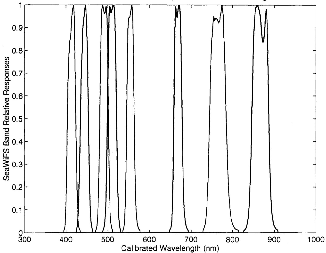
SeaWiFS In-Band Relative Responses at MOBY wavelengths
