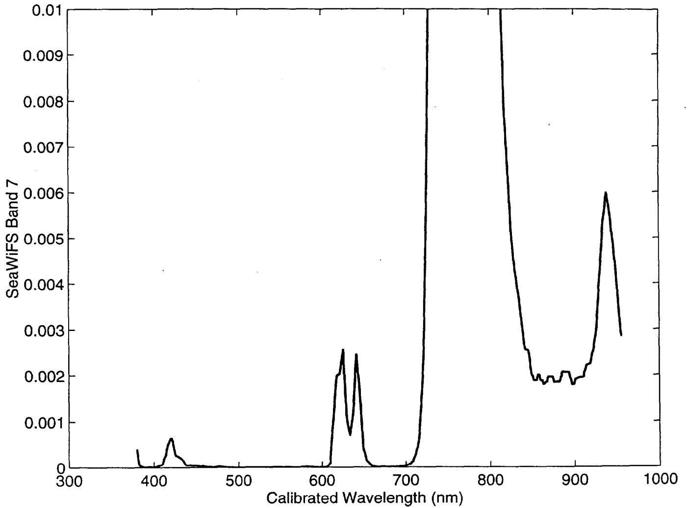
SeaWiFS Out-of-band Relative Responses at MOBY wavelengths
