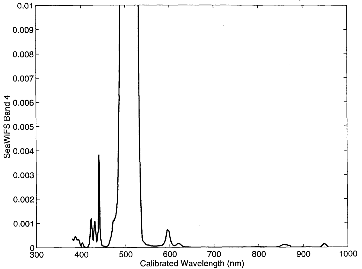
SeaWiFS Out-of-band Relative Responses at MOBY wavelengths
