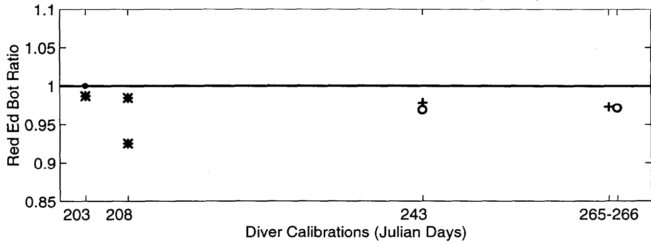
Diver Calibration - Ed Bot, SeaWiFS Band 6 (670 nm)
