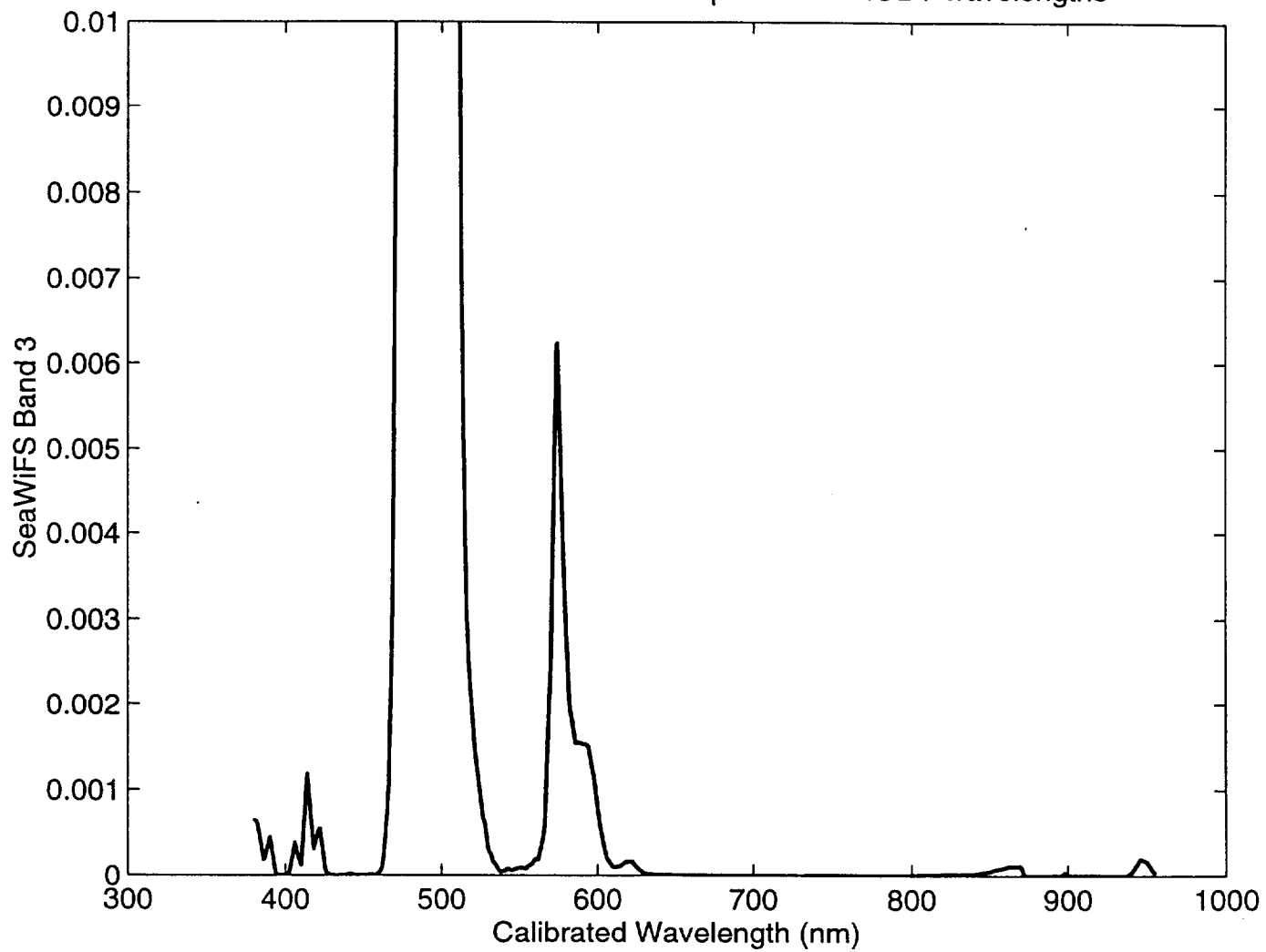
SeaWiFS Out-of-band Relative Responses at MOBY wavelengths
