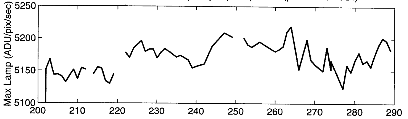
MOBY203, Maximum Lamp output (red spectrum, pixels 513:1024)
