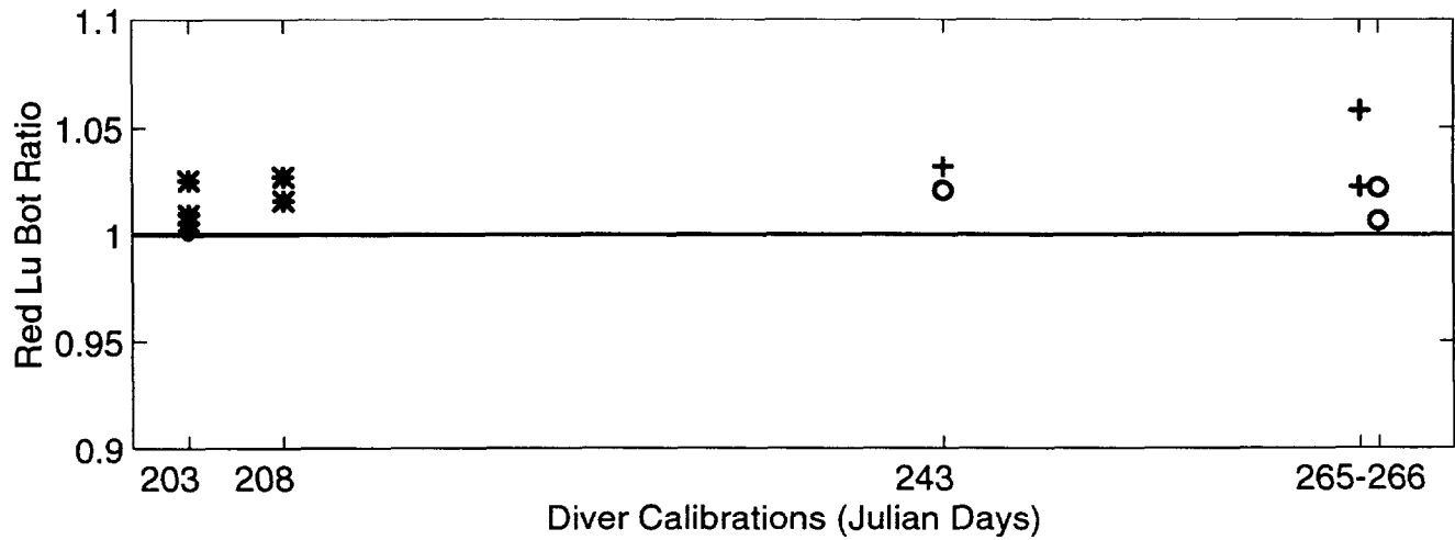
Diver Calibration - Lu Bot, SeaWifS Band 6 (670 nm)
